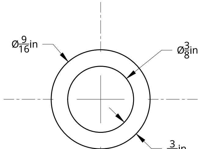
Front SCALE 3:1
